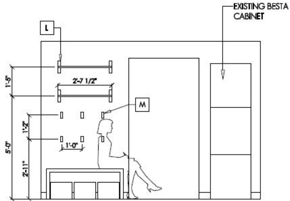
A TV WALL ELEVATION SCALE 1/4" = 1'-0"
