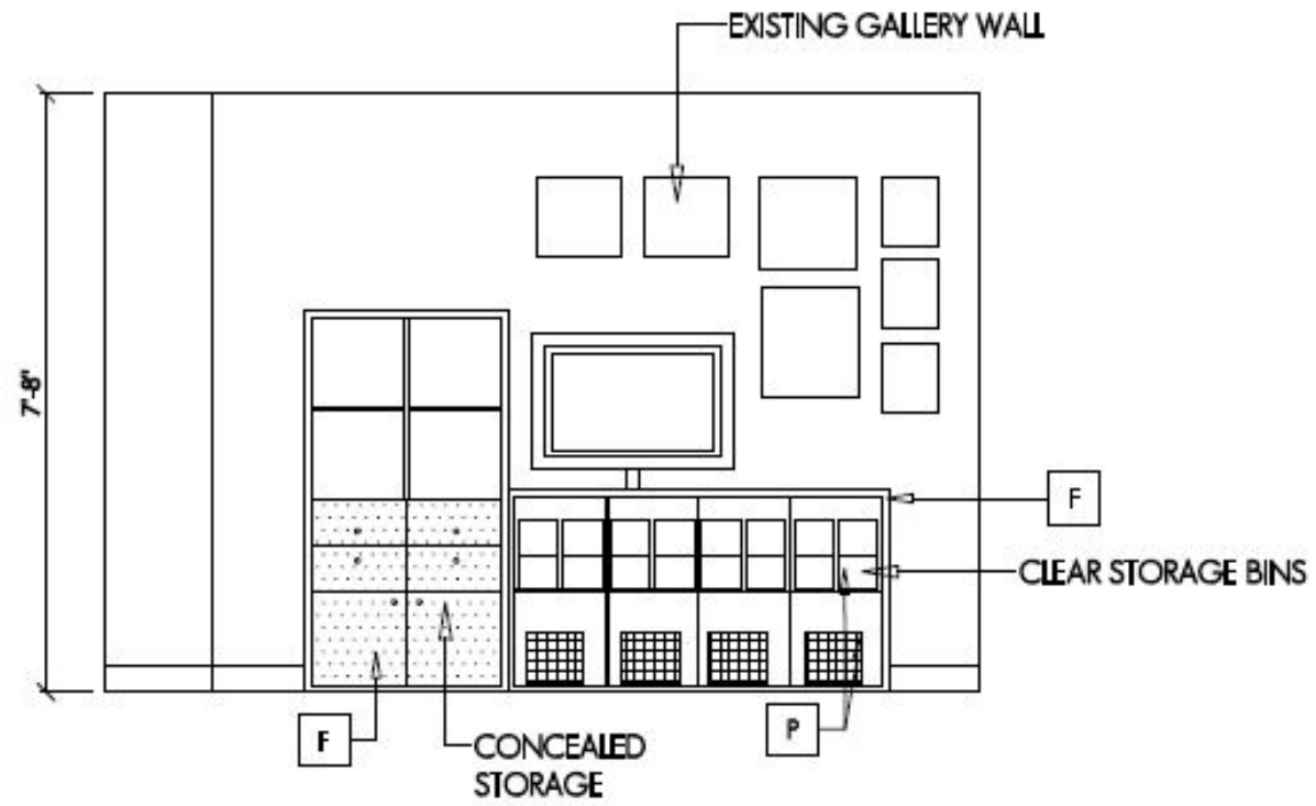
A TV WALL ELEVATION SCALE 1/4" = 1'-0"
